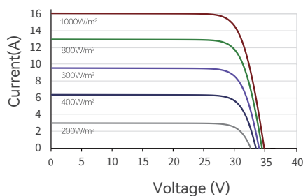
Current-Voltage(455W)
